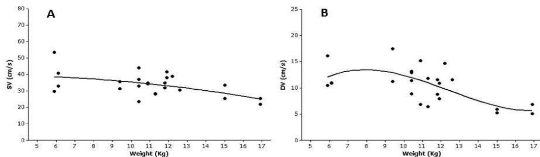
Figure 2. Graphic representation of the negative correlation between body weight of the animals and systolic velocity (SV; A) and diastolic (DV; B) of the adrenal glands in canines.
